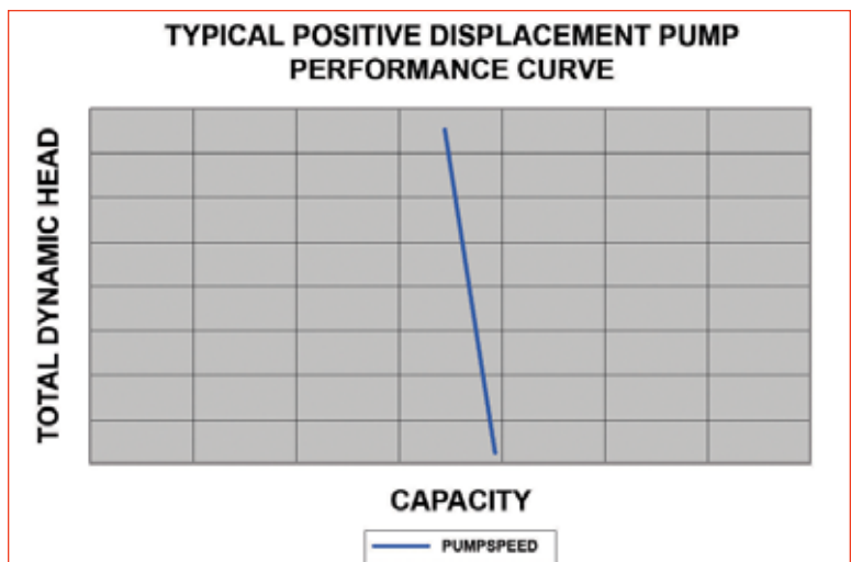
As total dynamic head increases (in feet), rotary lobe pumps are able to maintain an almost constant capacity (gpm) because they are positive displacement pumps.
