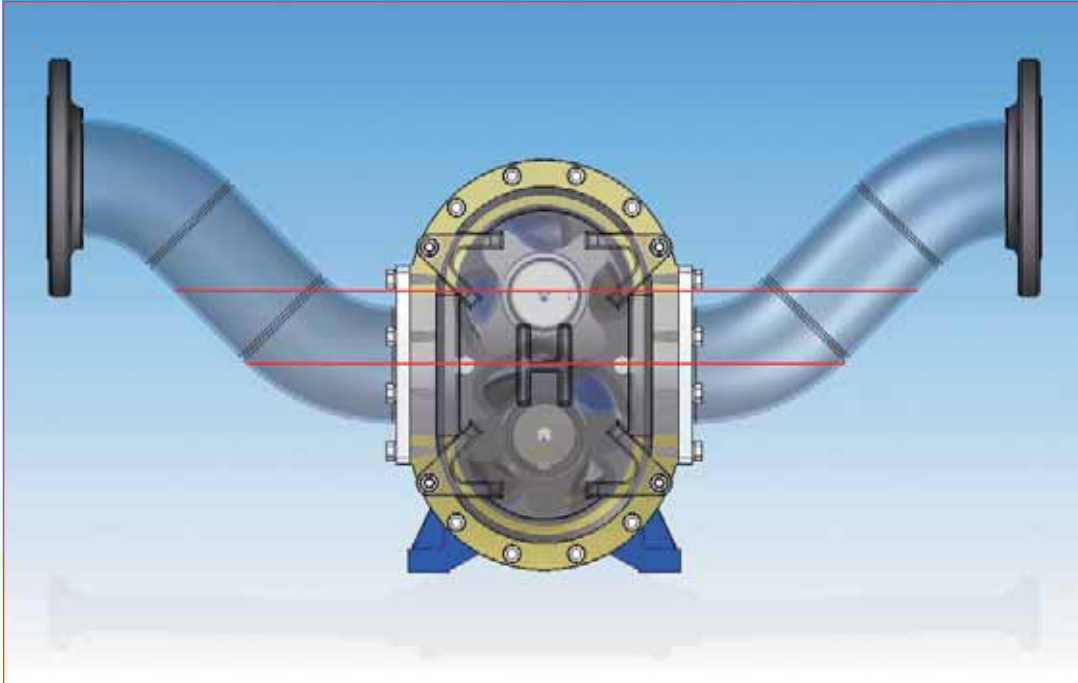
Suction and discharge piping configurations aid in priming rotary lobe pumps. Here, indicated in red, are typical fluid levels maintained within the quench chamber in order to assist priming.
