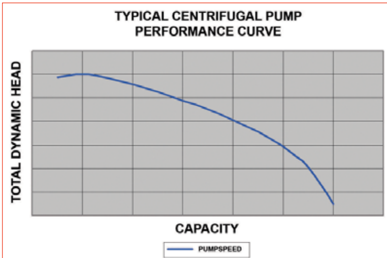
In a centrifugal pump, as total dynamic head increases (in feet), capacity decreases (gpm).
